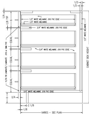
TYPICAL B0D4D INTEGRAL TOE KICK
