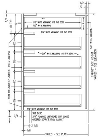
TYPICAL B0D5D FOR SUB BASE
