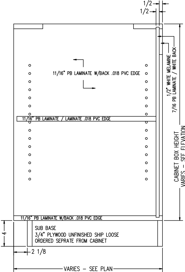
TYPICAL BOPEN FOR SUB BASE SCALE: 1-1/2" = 1'-0"
