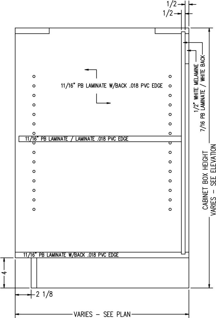
TYPICAL BOPEN INTEGRAL TOE KICK SCALE: 1-1/2" = 1'-0"
