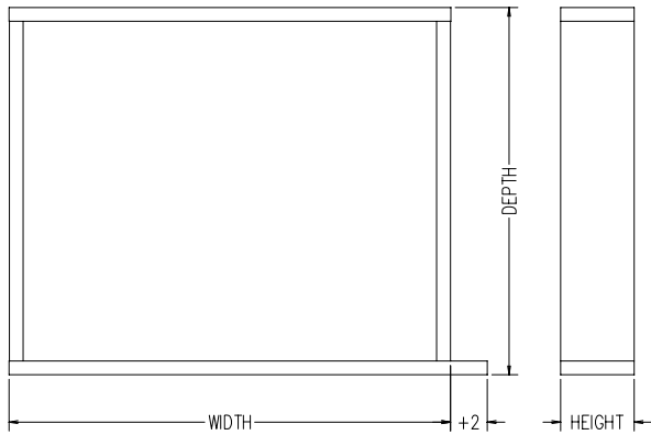
TYPICAL SUB BASE FINISHED LEFT SCALE: 1-1/2" = 1'-0"
