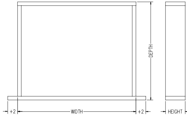
TYPICAL SUB BASE UNFINISHED LEFT & RIGHT SCALE: 1-1/2" = 1'-0"
