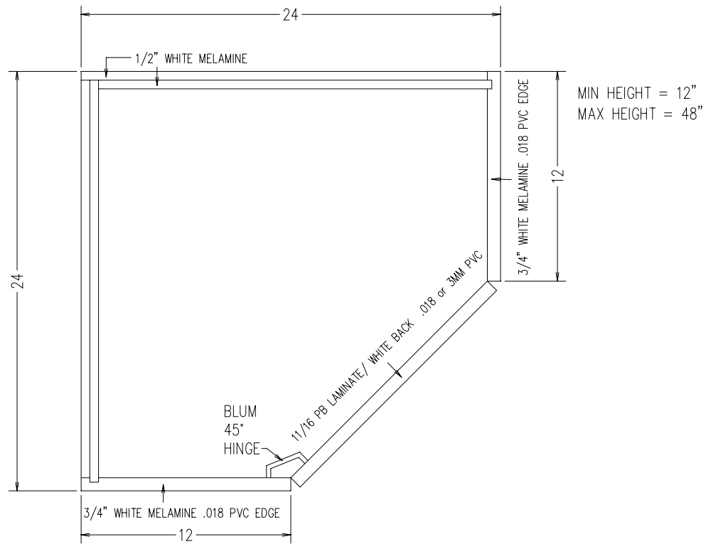
TYPICAL W1D-CORNER
