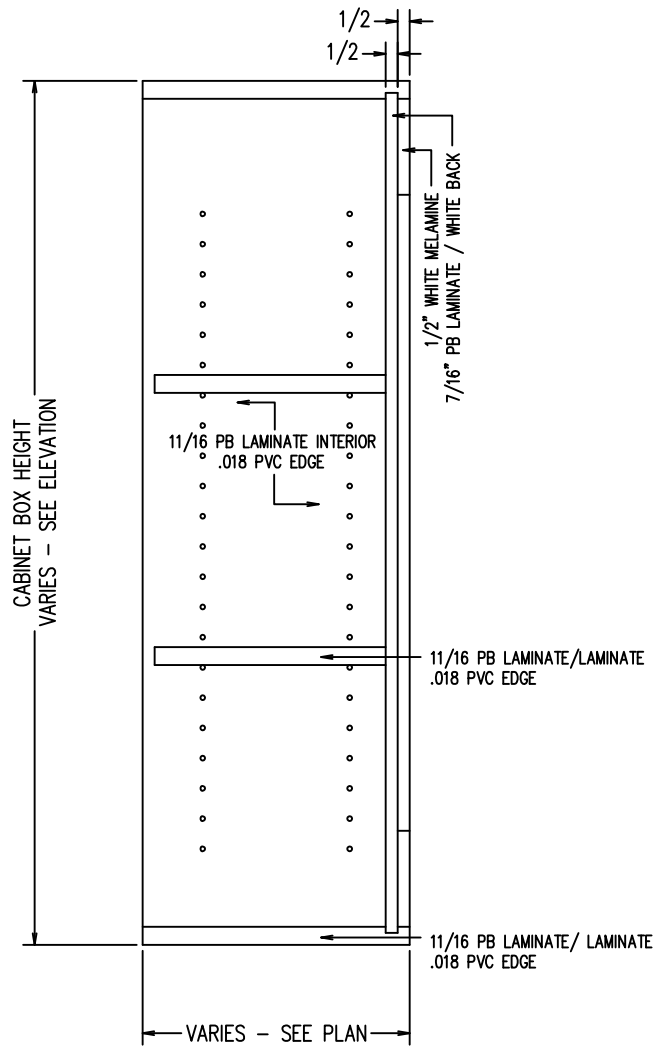
TYPICAL WOPEN W/OUT LIGHT RAIL SCALE: 1-1/2" = 1'-0"
