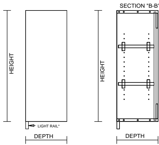
HANGING RAIL UNFINISHED END TYP.
