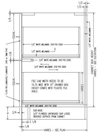
TYPICAL BOD2D FOR SUB BASE
