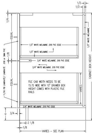
TYPICAL BOD2D INTEGRAL TOE KICK
